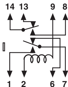
Figure R DPDT Without diode
